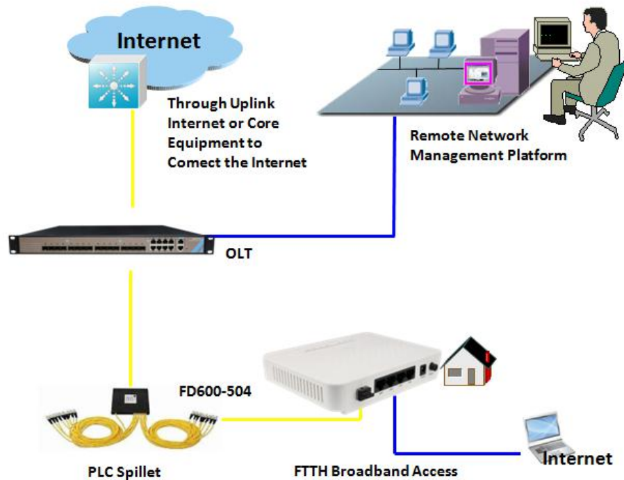
Figure: FD600-504 Application Diagram
