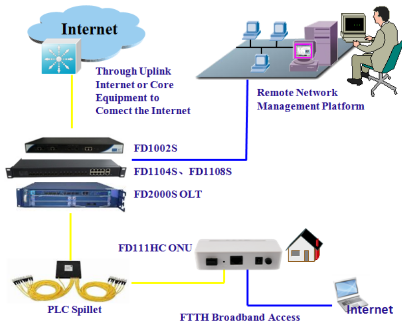
Figure: FD111HZ Application Diagram
