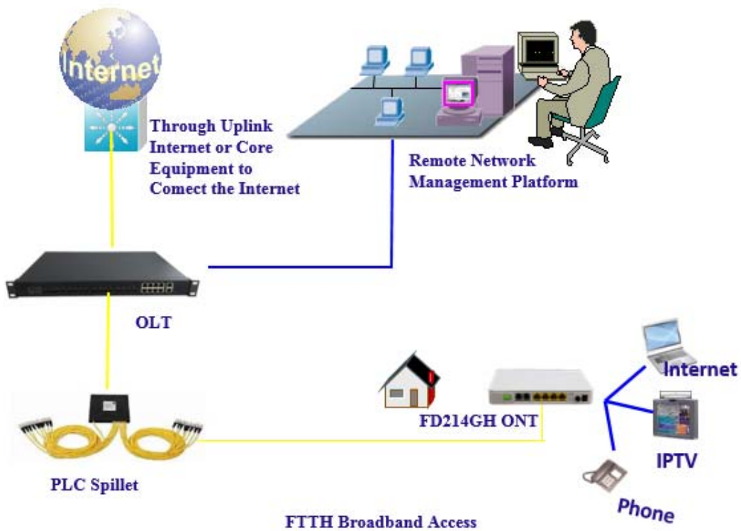
Figure: FD214GH Application Diagram
