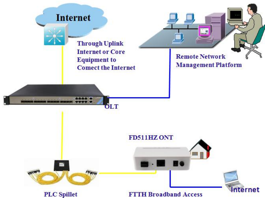
Figure: FD600-511G-HZ600 Application Diagram
