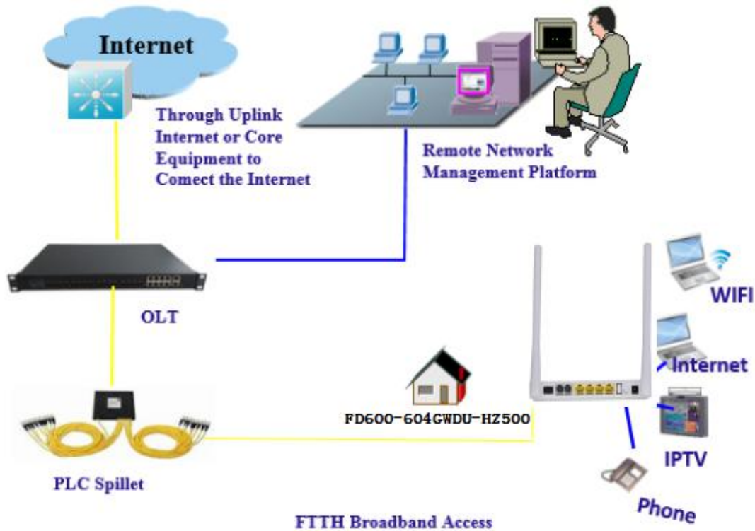
Figure: FD600-604GWDU-HZ500 Application Diagram
